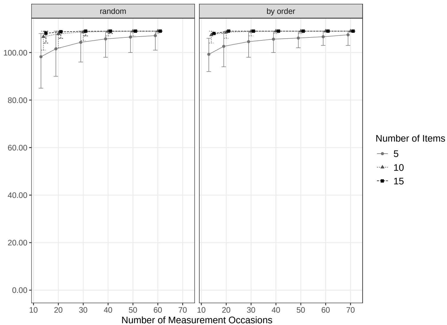
Number of ICCs for Reliability
